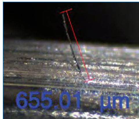
Fig. 28: Hair-like particle (tin whiskers) chipped off a tinned wire (655 μm long)
