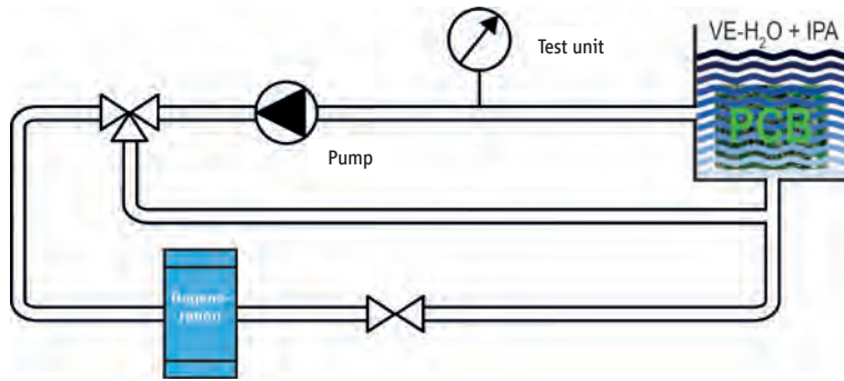
Fig. 105: Test procedure
