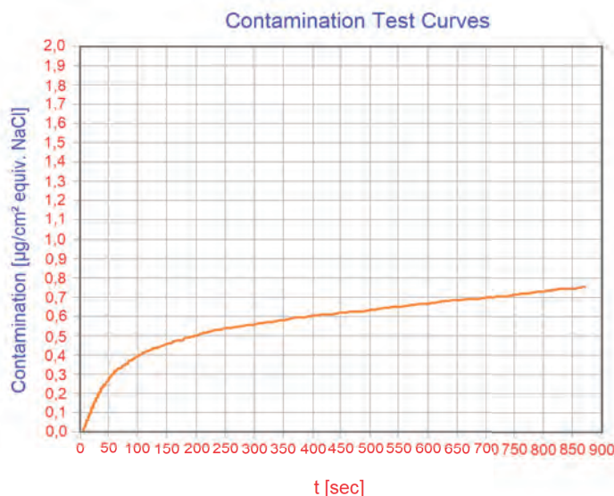
Fig. 106: Test curve
