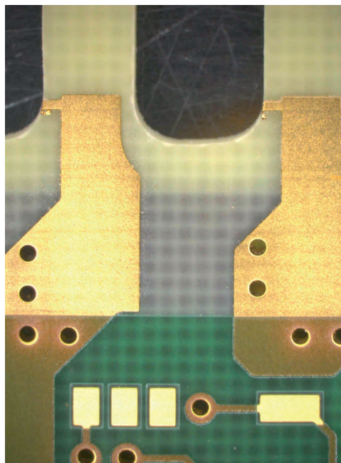
Fig. 61: Connections for electroplated gold areas
